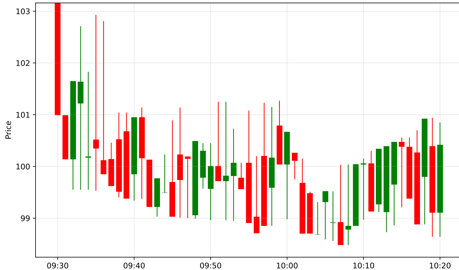
Simulation Run: Price Action (1-Min OHLC)
